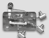
S840 v Roller lever, short and captive screws
