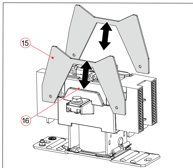
Fig. 41: C195 X/: Removing the pole plates
