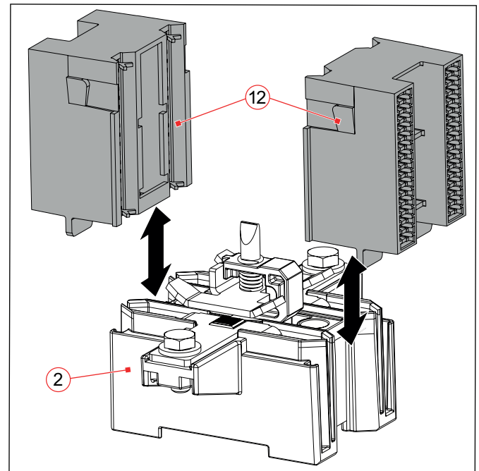
Fig. 51: C195 X/: Removing/attaching the arcing chambers
