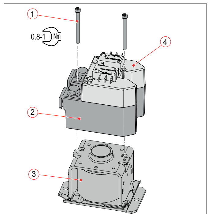
Fig. 57: C195 S/, C195 T/: Disassembling/assembling the contact unit (the figure shows C195 S/, the procedure is identical for C195 T/)
