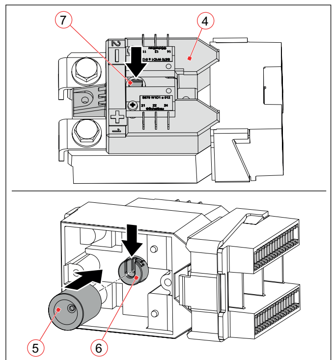
Fig. 62: C195 A/, C195 B/: Assembling the armature (the figure shows C195 A/, the procedure is identical for C195 B/)
