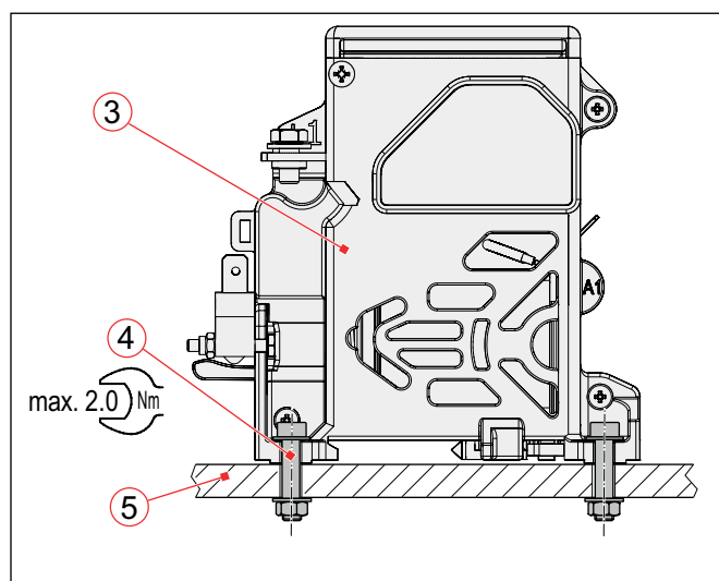
Fig. 7: Install the contactor to the mounting plate (the figure shows the C193 series, the procedure for the C294 series is the same)
